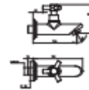
Bib Cock with Wall Flange G1916A1
